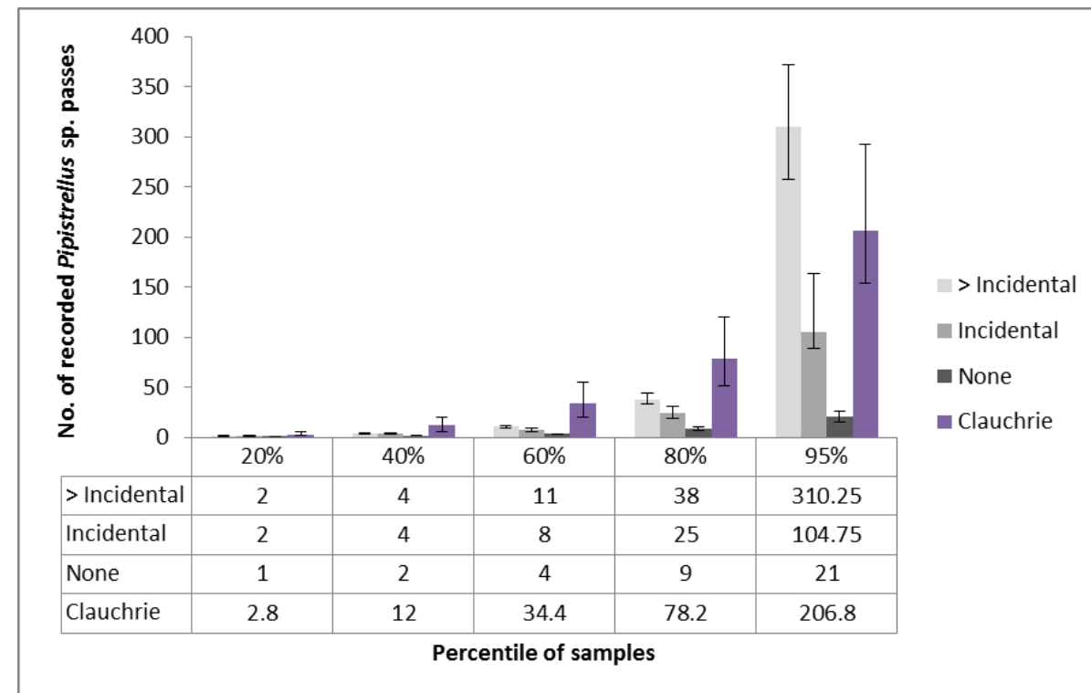
Figure 2: Number of pipistrelle bat passes per night at WTG4 at different percentiles compared to operational projects with a known category of bat fatality. Error bars are 95 % CIs derived using bootstrap methods due to non-normal distribution of the datasets.
