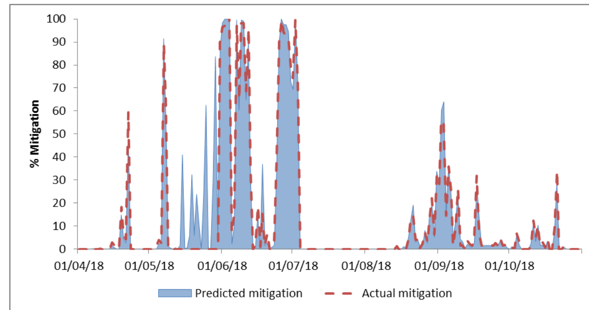
Figure 5: Example output of the auditing available from turbine SCADA data for another SPR windfarm in 2018. The blue shaded areas show the predicted mitigation (based on weather data) and the red dashed line shows the actual mitigation implemented during each night automatically by the CORE software. Data not available during two periods of site outage 9-29 th May and 5 th July – 12 th August, when turbines were non-operational.
