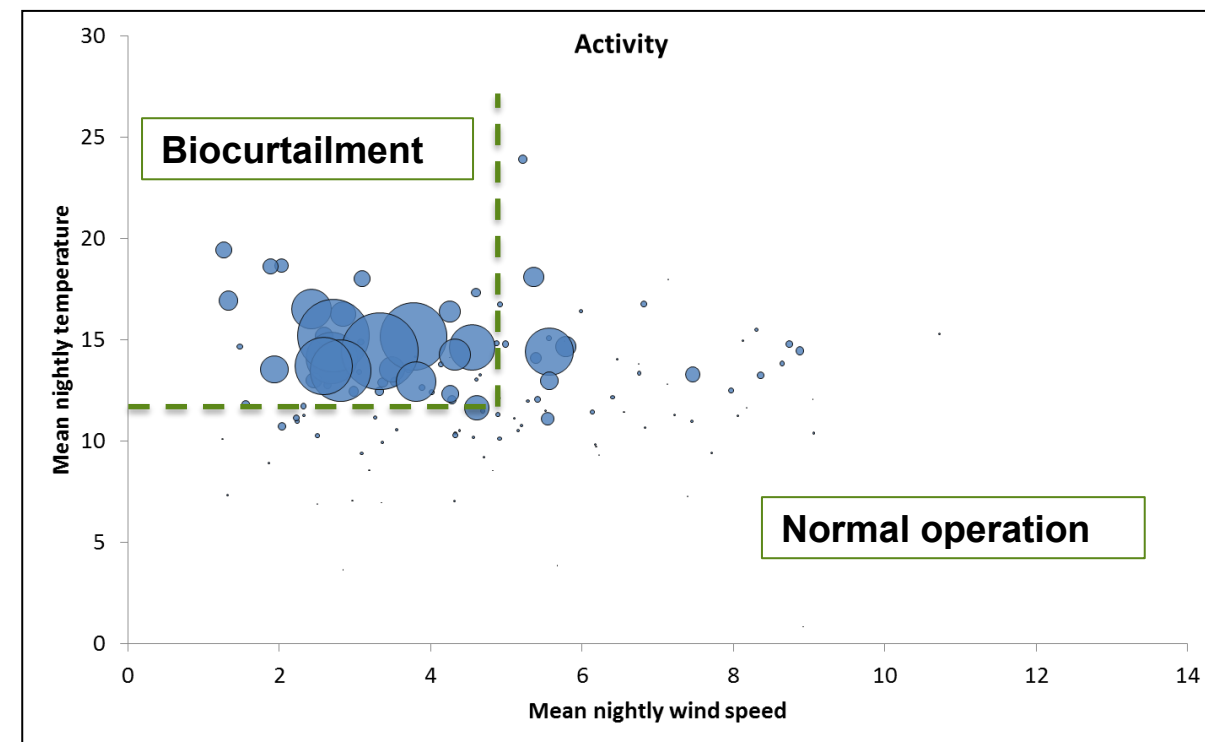
Figure 3: Typical pattern of bat Pipistrelle activity compared to wind speed and temperature parameters measured at upland operational windfarms in south-west Scotland. The dashed lines indicate the 5 m/s wind speed and 11.5 degrees C thresholds which correspond with circa. 90% of all activity.
