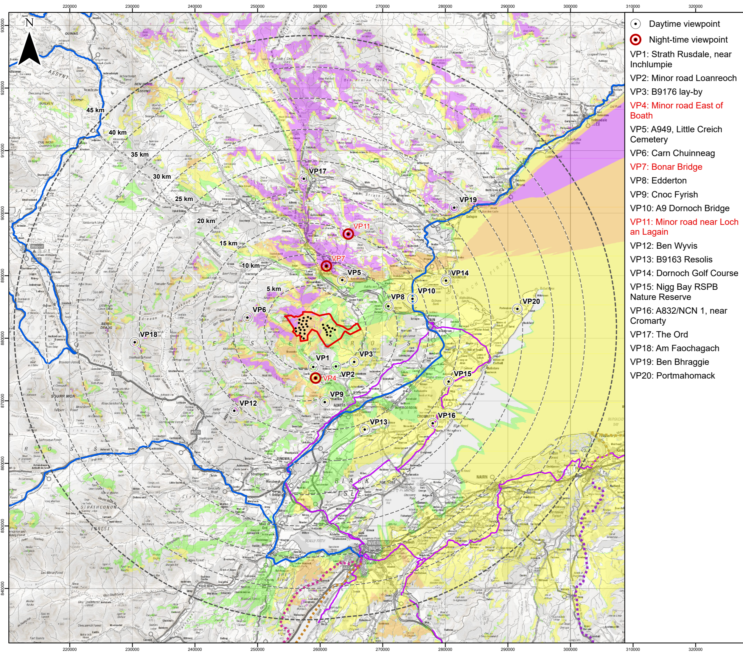
Figure 4.2a: Blade Tip Height ZTV (180 m) and Visual Receptors - 45 km
