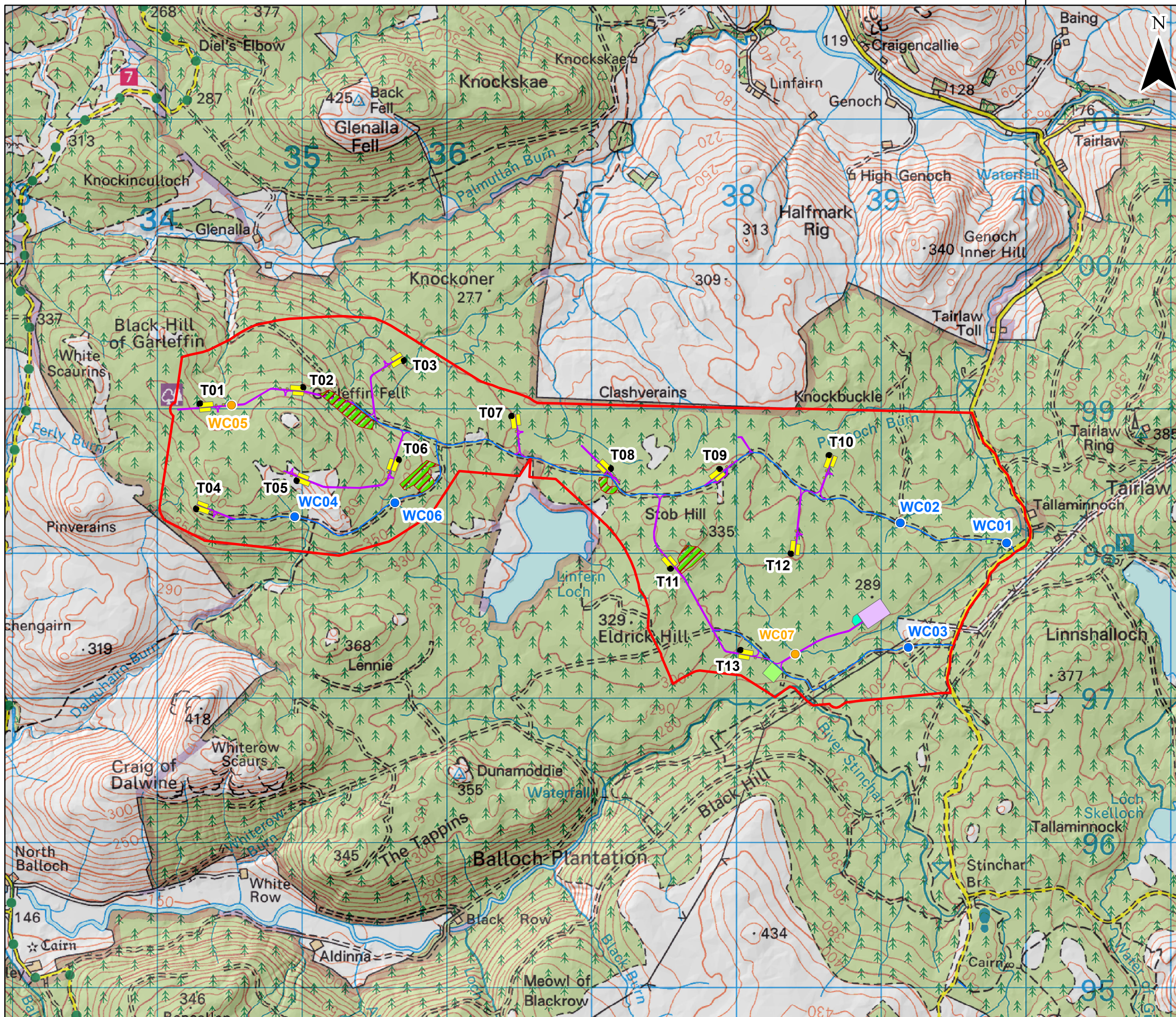
Carrick Windfarm Figure 4.1: Site Layout
