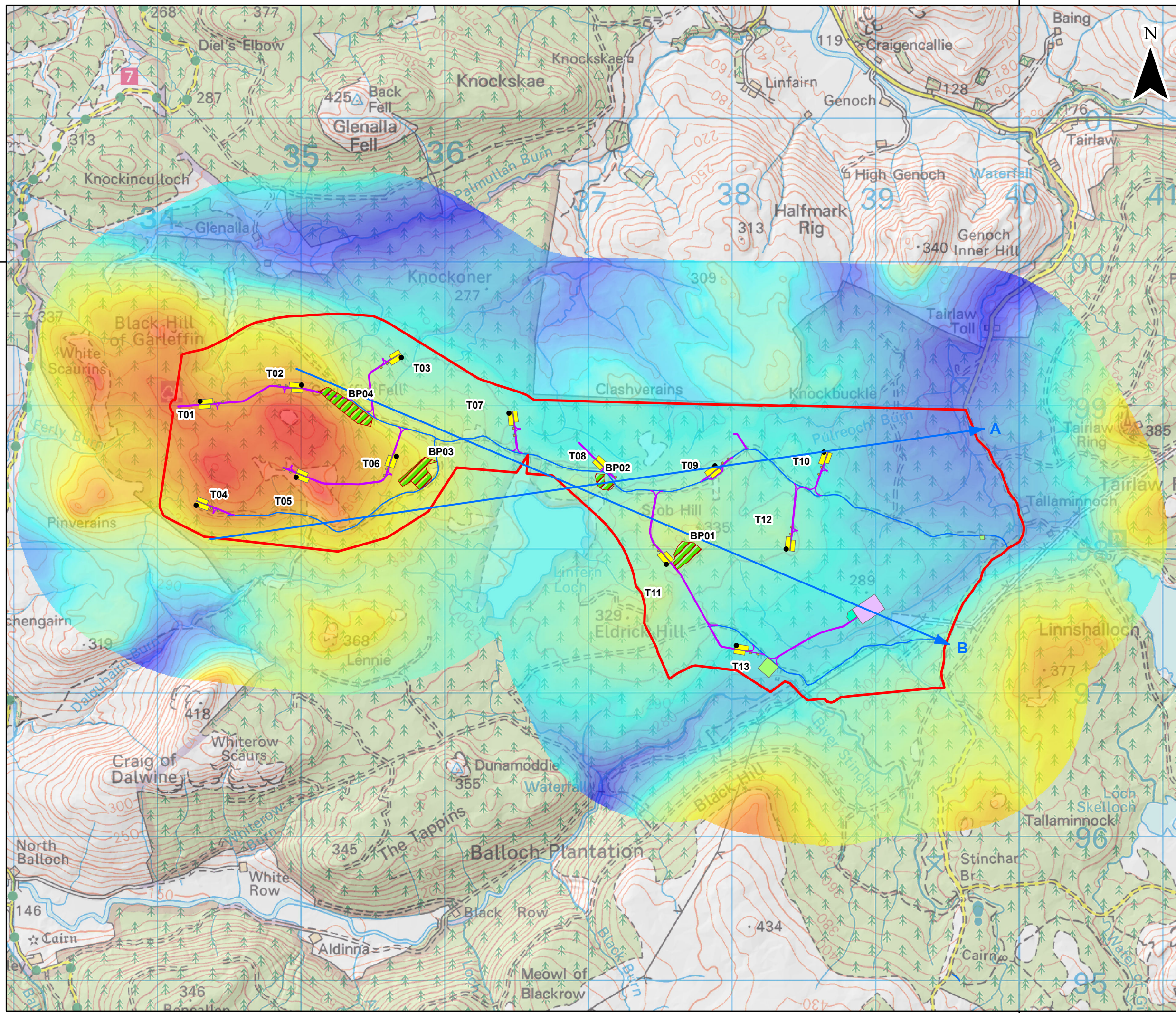
Carrick Windfarm Figure 6.1: Elevation
