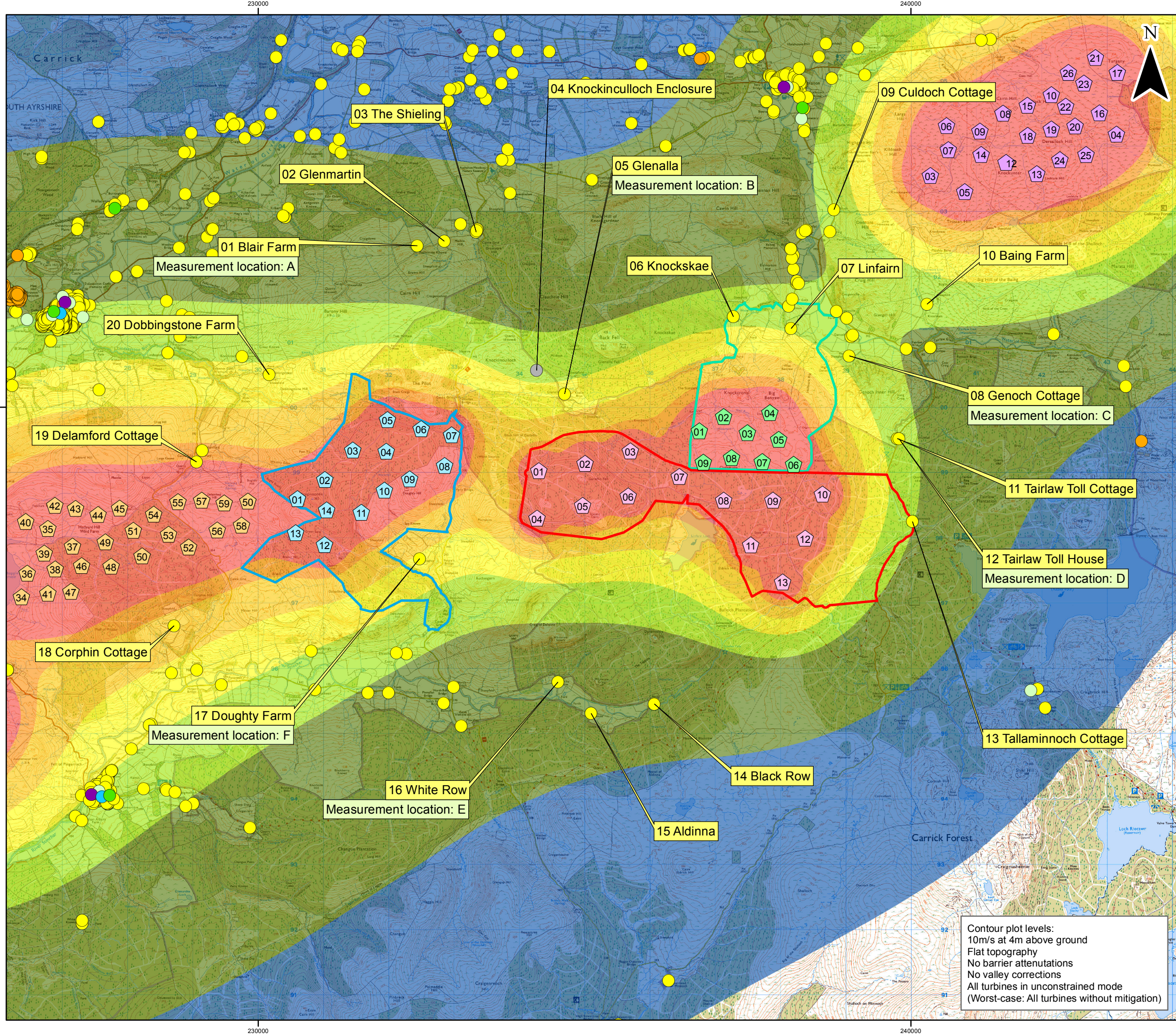
Carrick Windfarm Figure 9.3: Noise Contour - 10m/s - All Cumulative Developments (Operational and Proposed)
