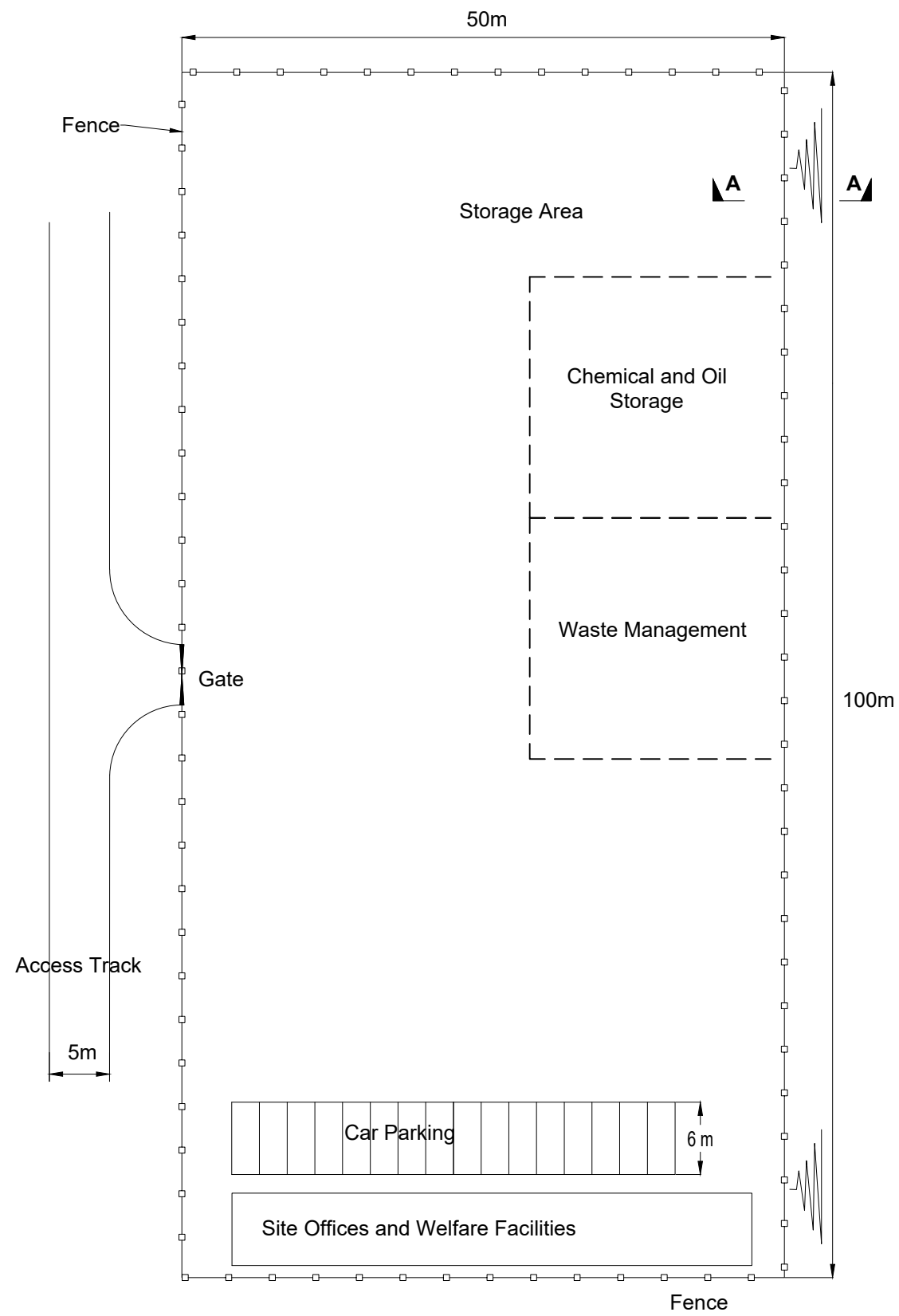
Typical Construction Compound
