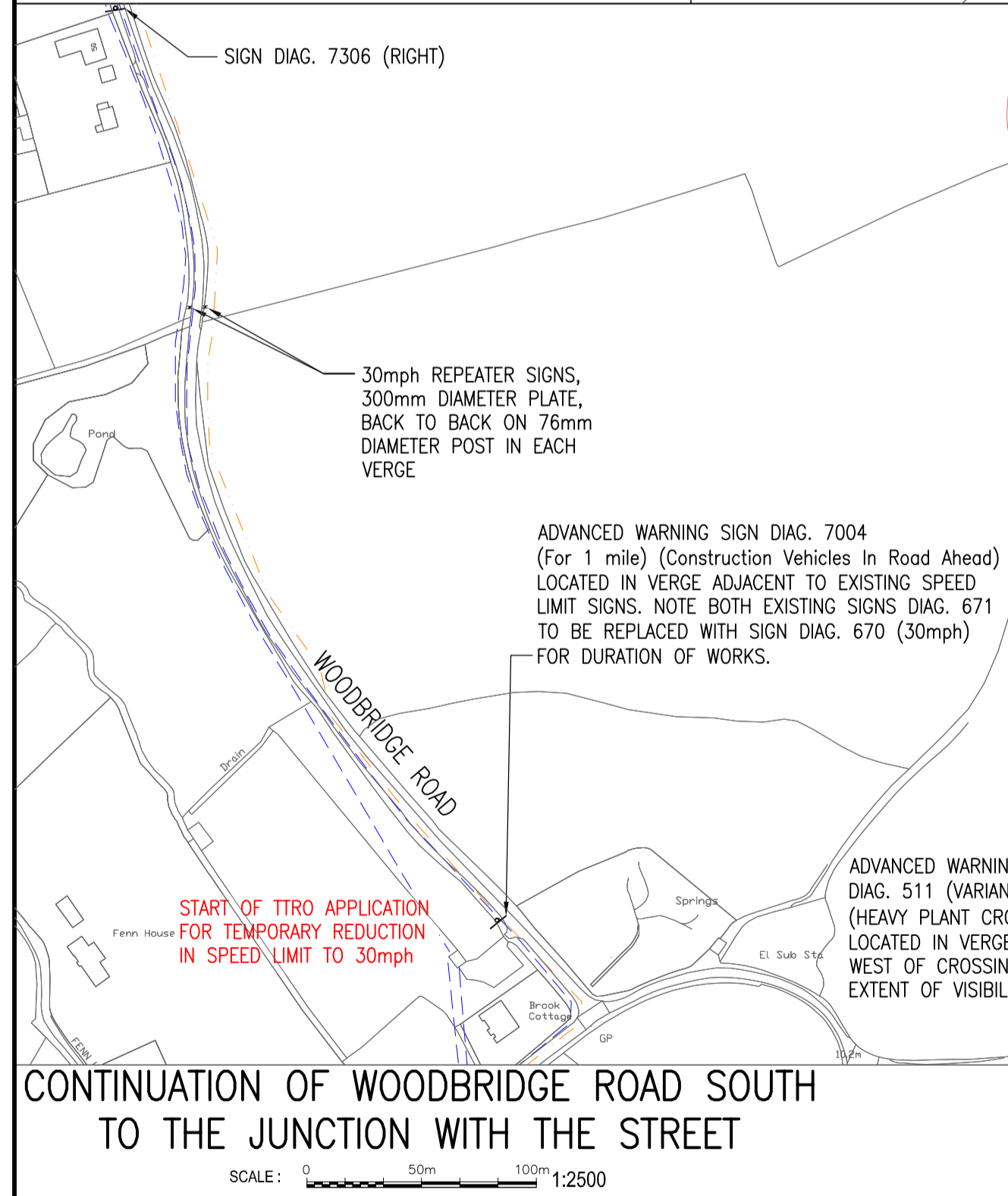
LOCATION PLAN FOR ACCESS AP-I INDICATING ADVANCE WARNING SIGNAGE SCALE: 0 50m 100m 1:2500
