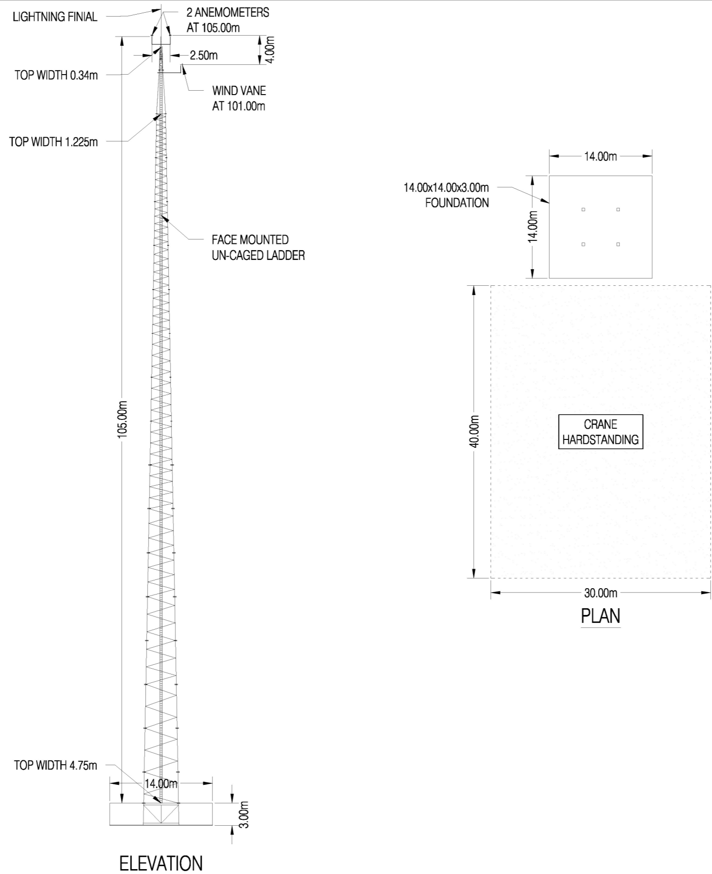
Harestanes West Windfarm Figure 3.12: Indicative Permanent Meteorological Mast
