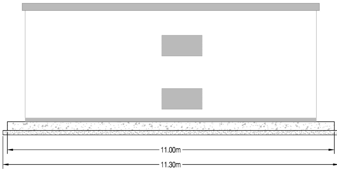
REAR ELEVATION
