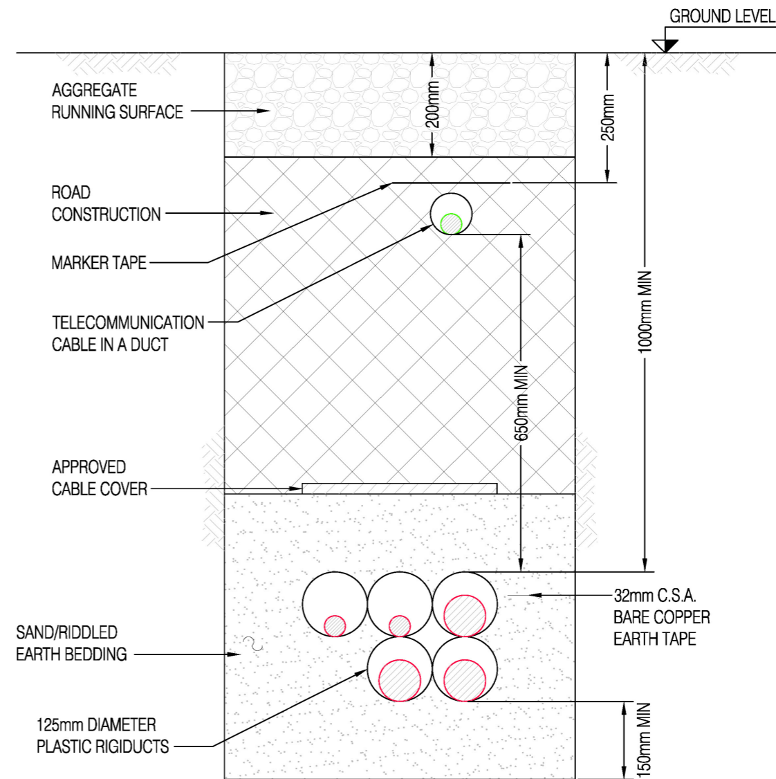
3-33kV CABLES ROAD CROSSING
