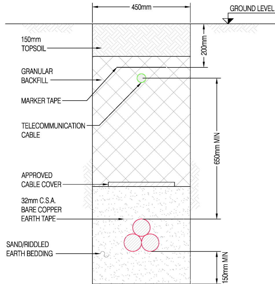
3-33kV CABLES IN TREFOIL FORMATION
